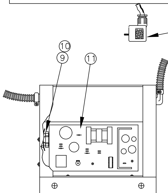
POWER SUPPLY BOX
